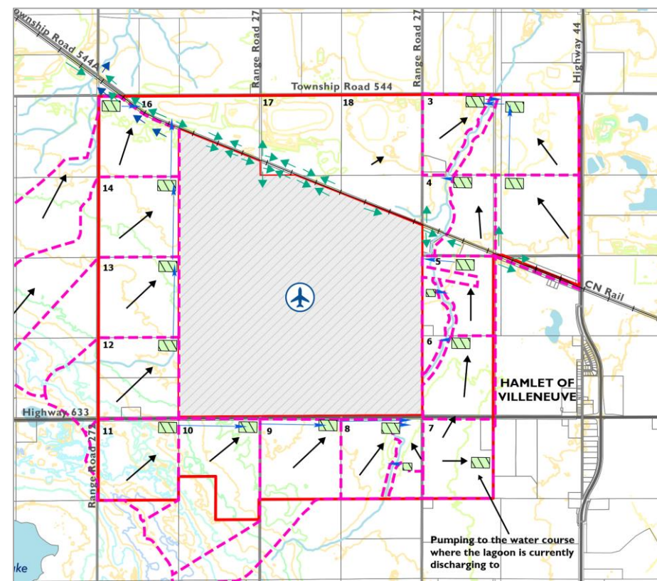
Figure 10 - Stormwater Management System
