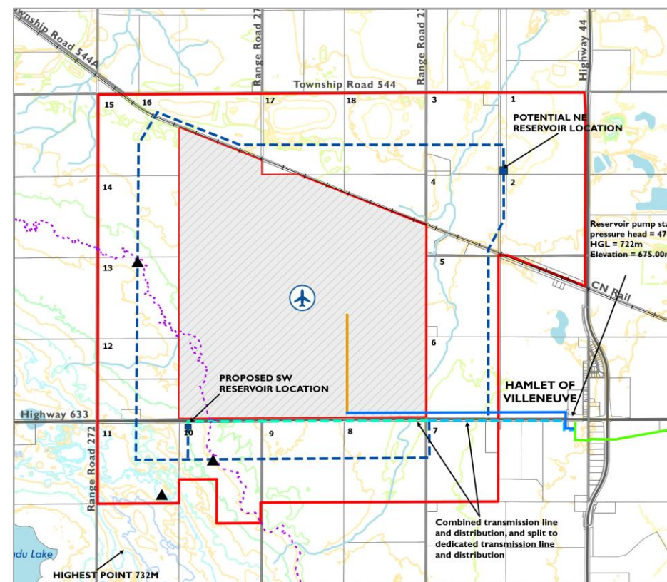
Figure 9 - Potable Water System
