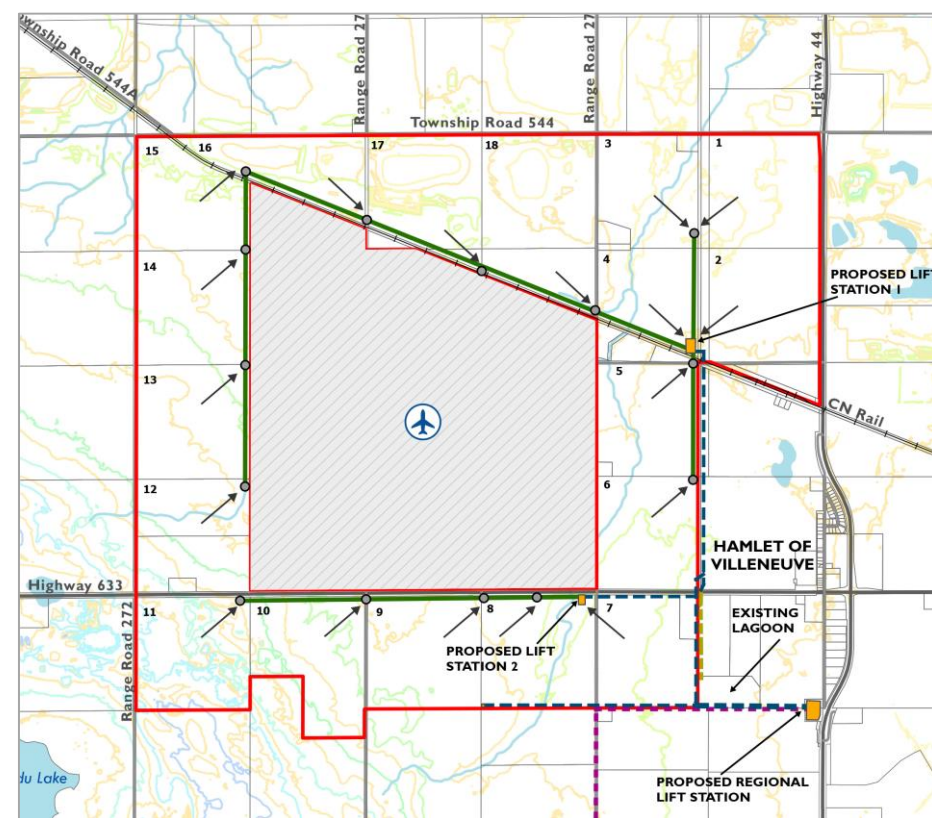
Figure 8 - Sanitary System
