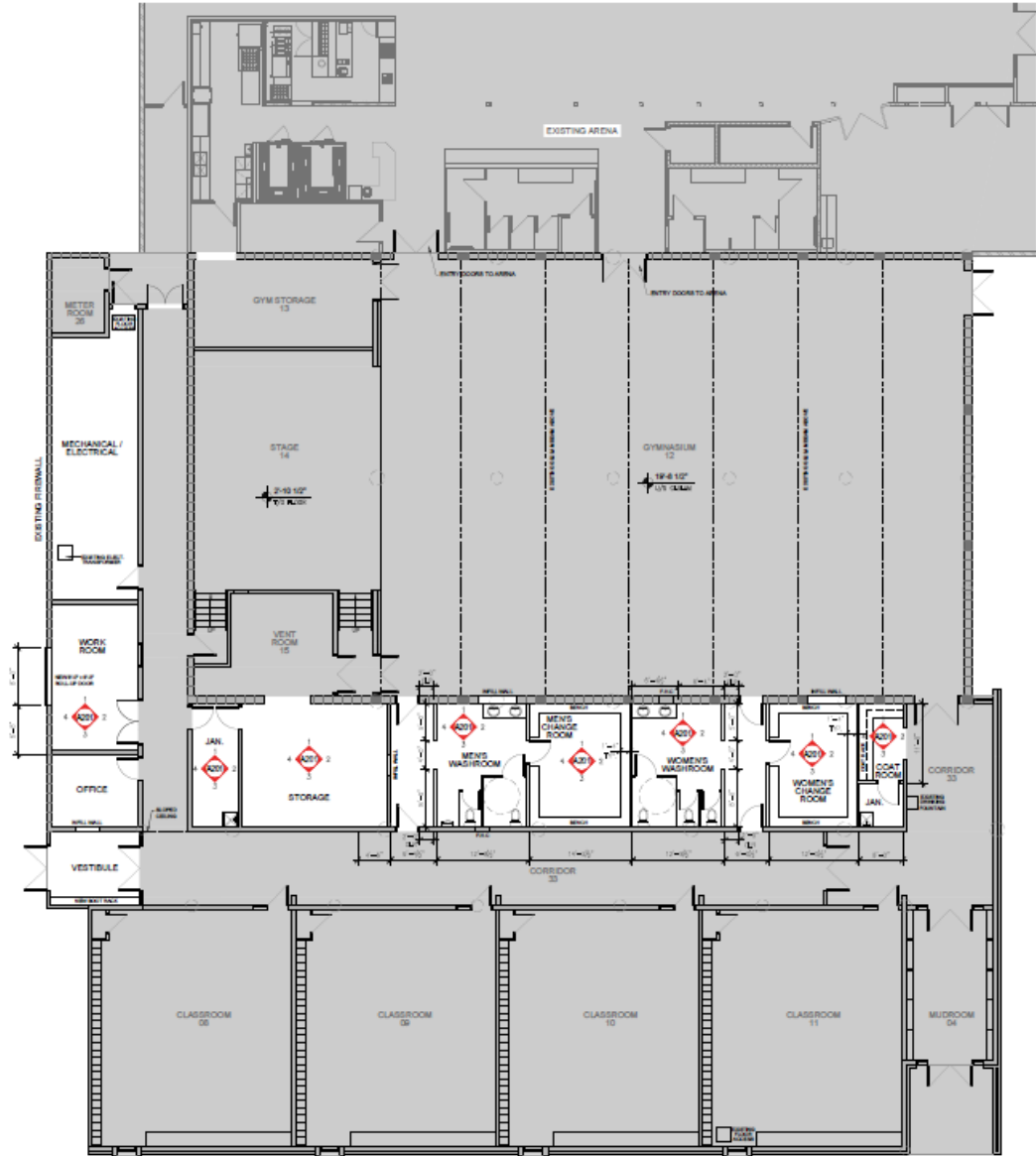
MAIN FLOOR PLAN 1/8" = 1'-0"
